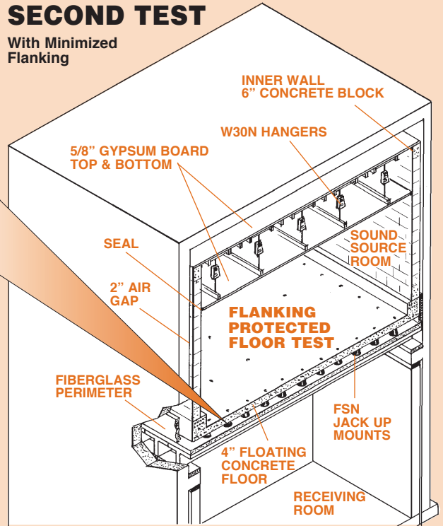
SECOND TEST JUNE 1971 OF SAME FLOATING FLOOR WITH ISOLATED WALLS AND CEILING TO PREVENT FLANKING. BASICALLY ROOM WITHIN A ROOM CONSTRUCTION.
