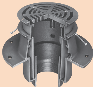
Type CFDA4 x 4 FLOOR DRAIN
