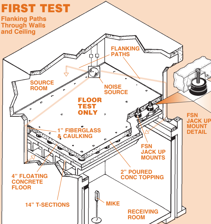
FIRST TEST MARCH 1971 OF A FLOATING FLOOR ONLY. DISAPPOINTING RESULTS BECAUSE OF FLANKING PROBLEMS DOWN THE WALLS.
