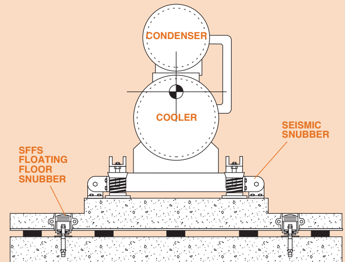
SNUBBER SHOWN WITH EAFM PANEL SYSTEM Equally suitable for FSN Jack-Up Floors
