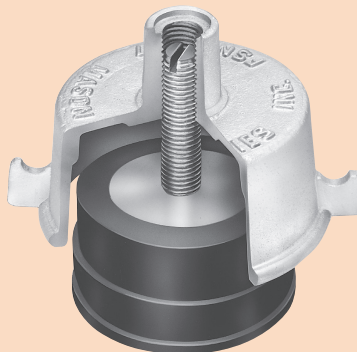
Type FSN LDS JACK-UP MOUNT
